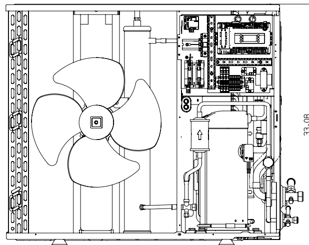
VIEW WITHOUT COVER FRONT LEFT, GUARD FAN & DOOR ASSM ⑦
