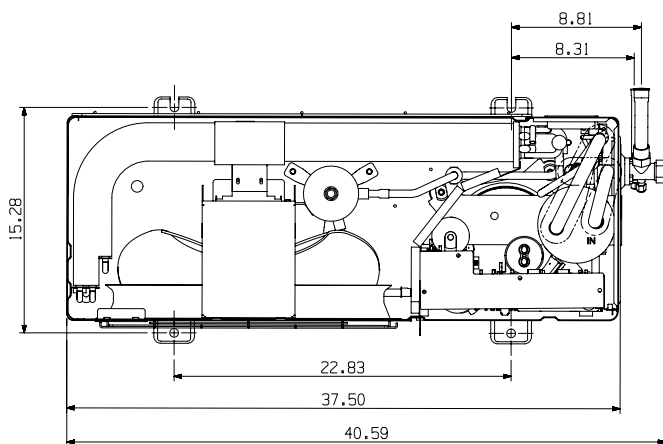
VIEW WITHOUT COVER TOP ⑥
